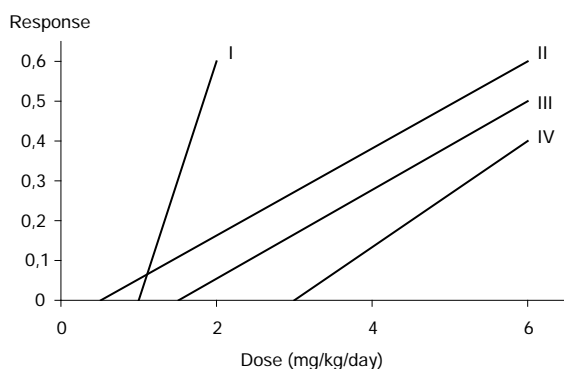
Figure 2. Hypothetical dose-response curve for four compounds I, II, III and IV.
